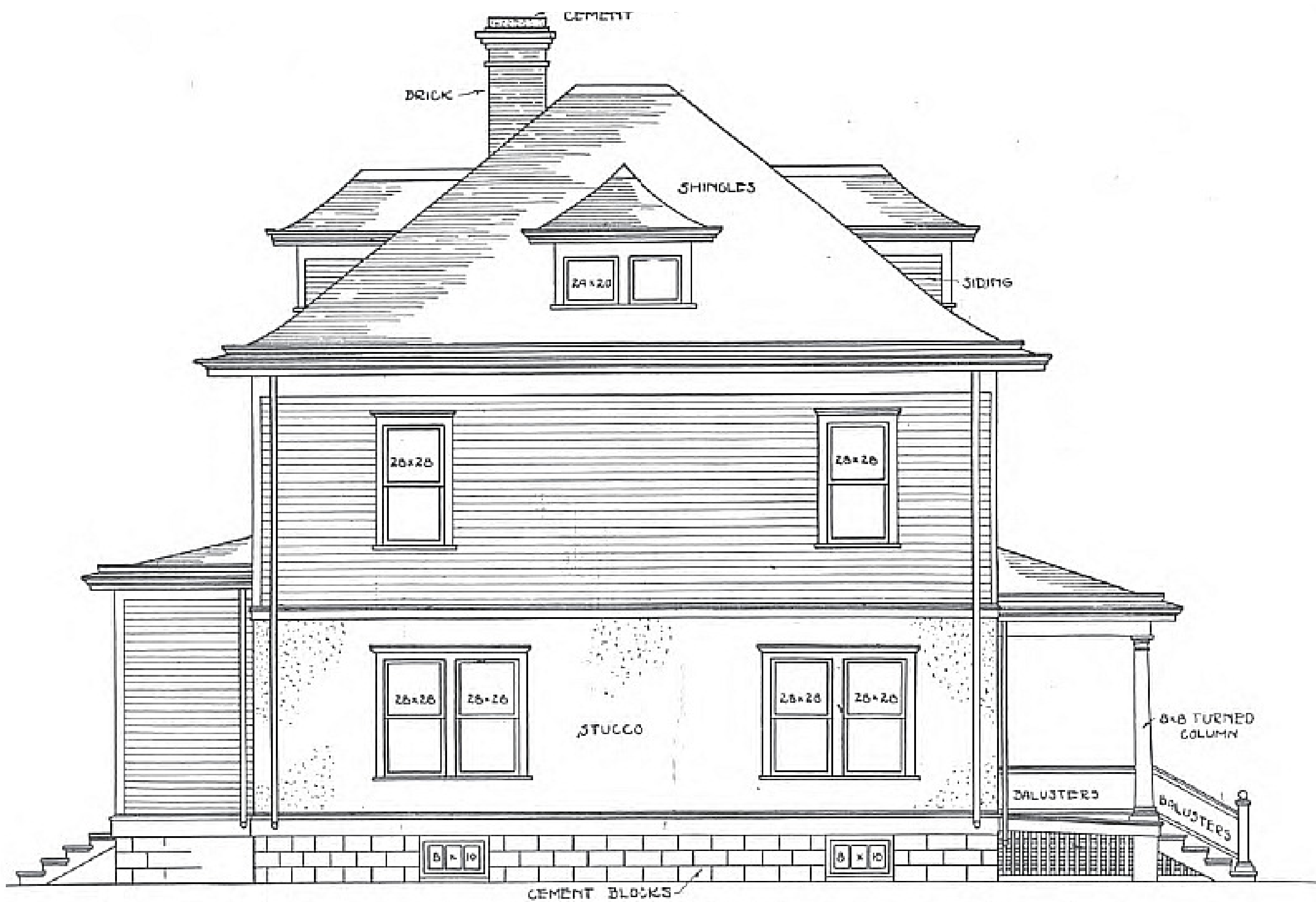
LEFT SIDE ELEVATION SCALE 3/4\"/>
