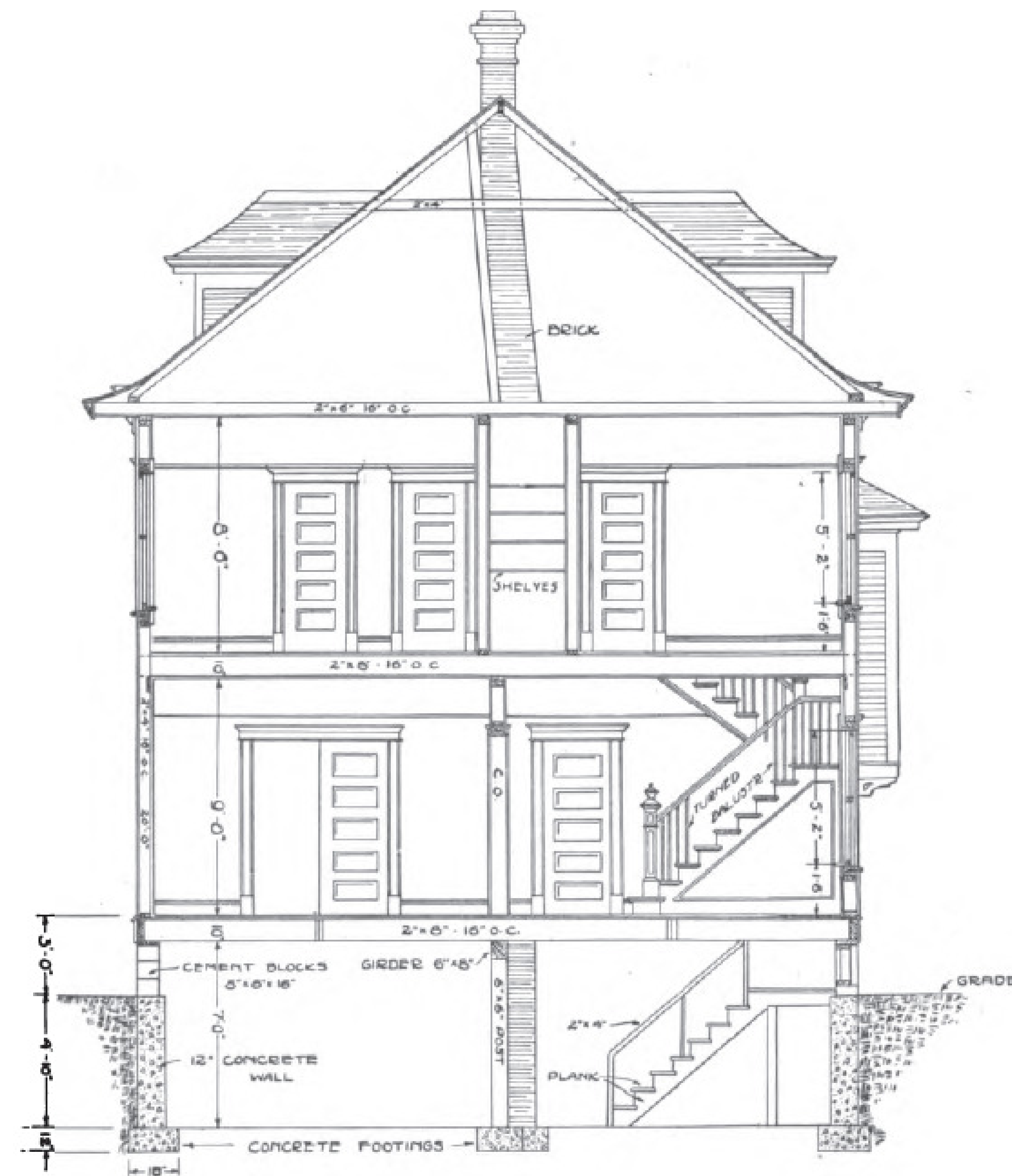
SECTION ON LINE AA
